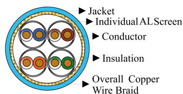
Cat7 S/FTP
